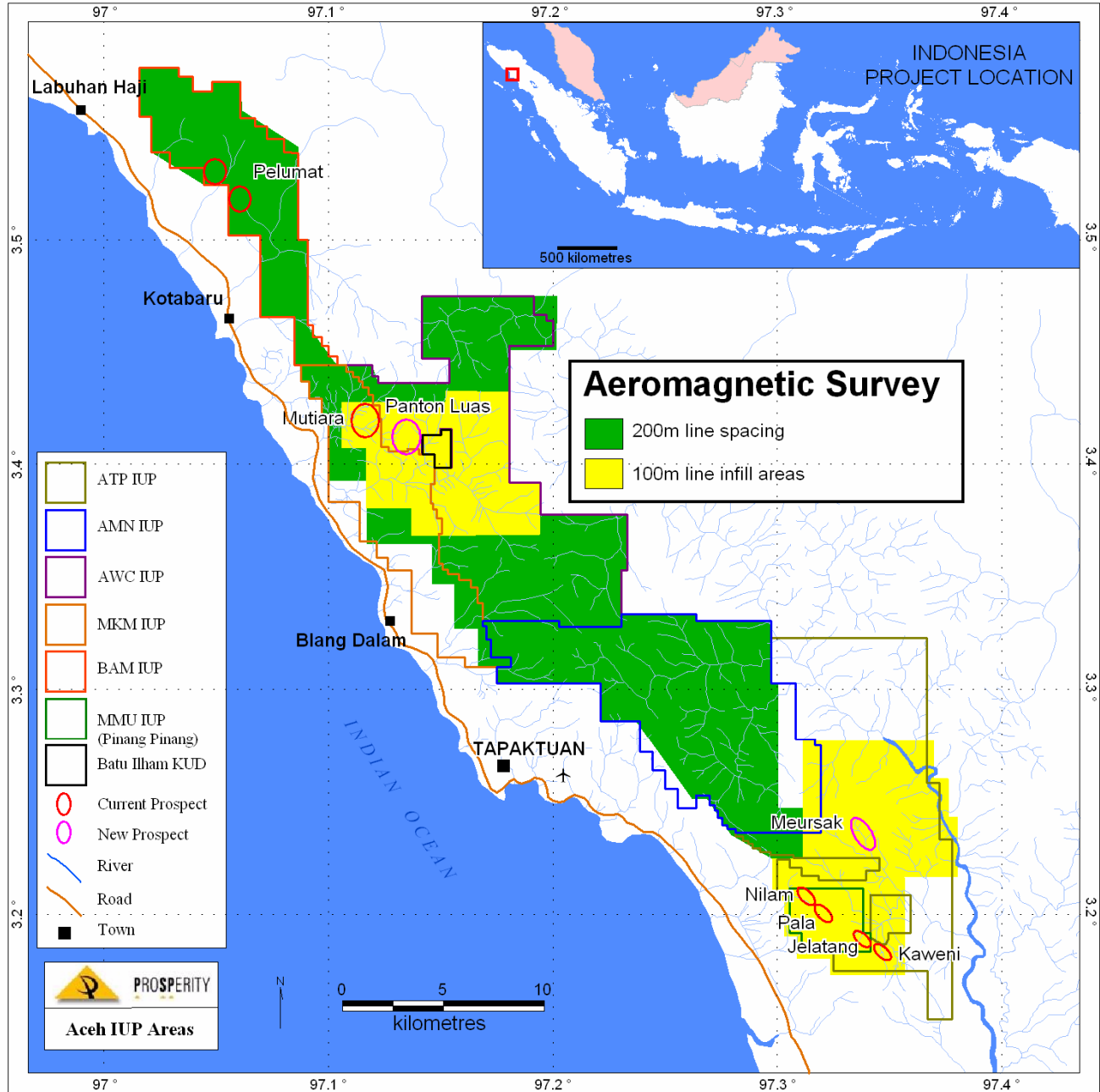
Location Map: Prosperity's Aceh IUPs and aeromagnetic survey
